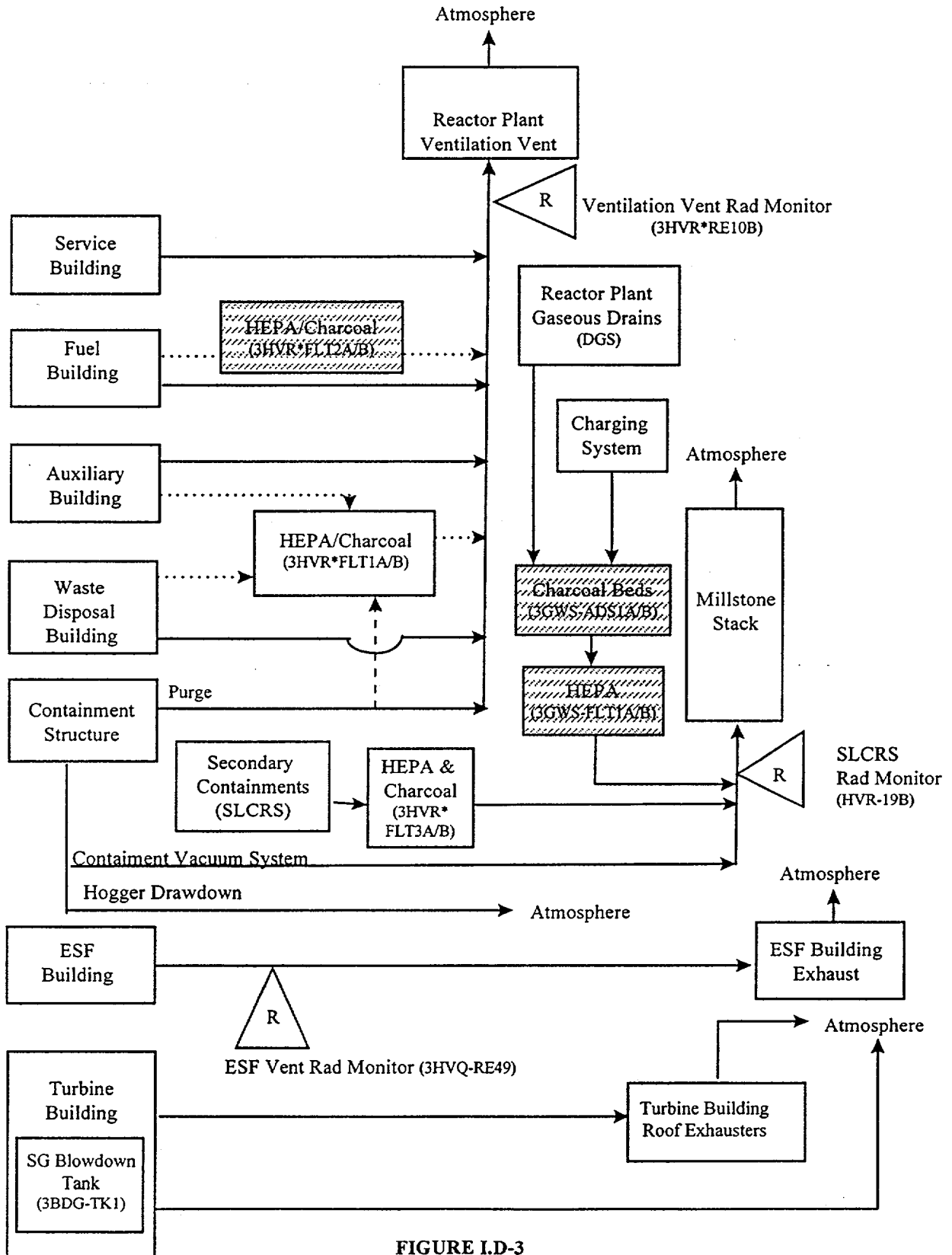
FIGURE I.D-3 SIMPLIFIED AIRBORNE EFFLUENT FLOW DIAGRAM MILLSTONE UNIT THREE
