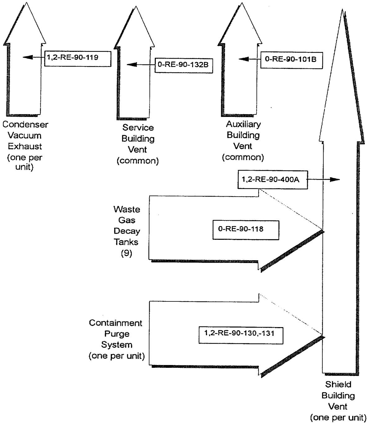
Figure 7.1 - GASEOUS EFFLUENT RELEASE/DISCHARGE POINTS
